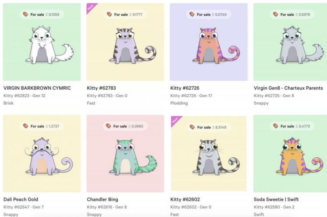
Slika 6. CryptoKitties platforma
